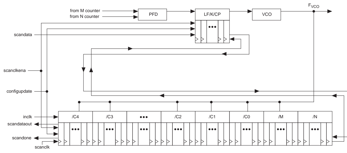
Figure 5–20. PLL Reconfiguration Scan Chain
