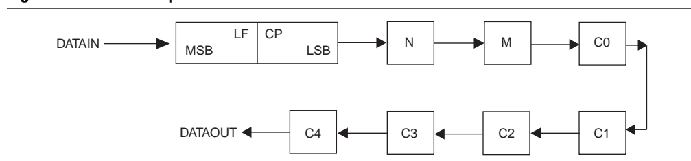
Figure 5-22. PLL Component Scan Chain Order
