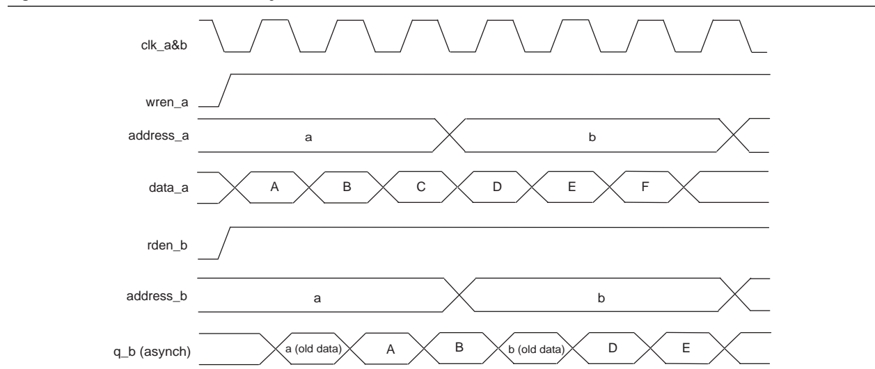
Figure 3-17. Mixed Port Read-During-Write: Old Data Mode
