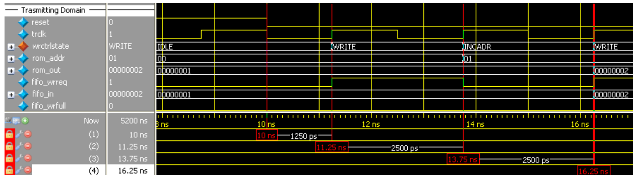
Figure 7. Initial Write Operation to the DCFIFO Megafunction
