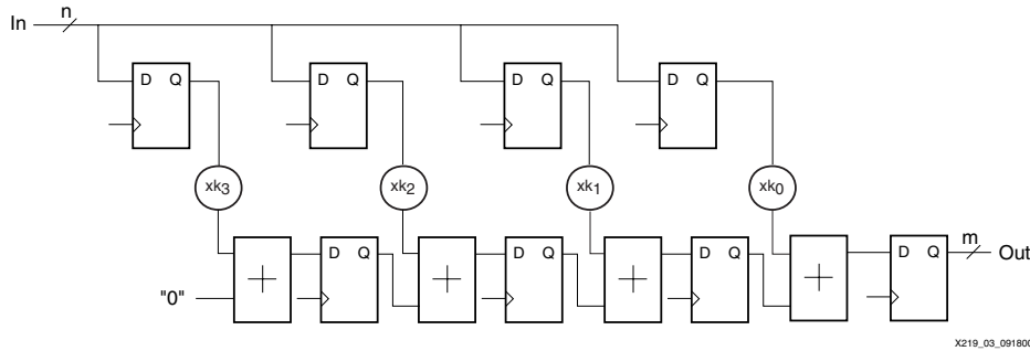
Figure 3: Transposed Form FIR Filters Employing Cascaded Pipelined Adders
