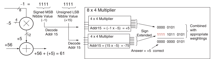
Figure 5: KCM Implementation with Two ROM Tables
