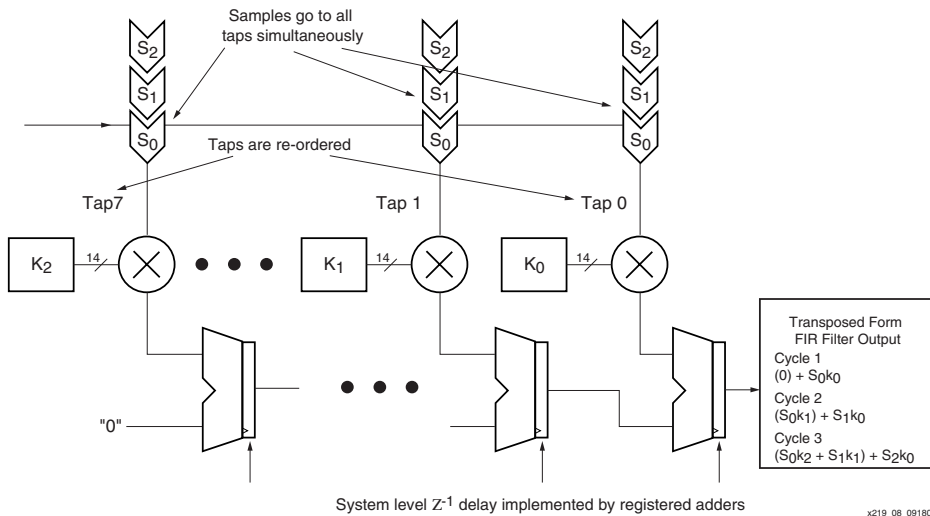
Figure 8: Transposed Form FIR Filter Block Diagram
