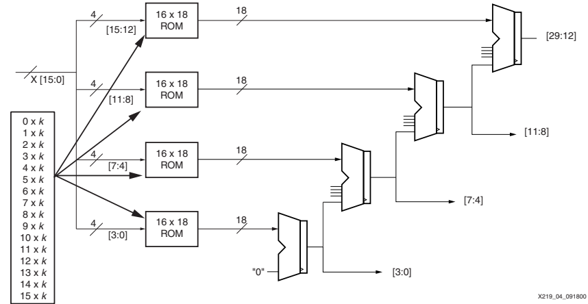
Figure 4: KCM Block Diagram
