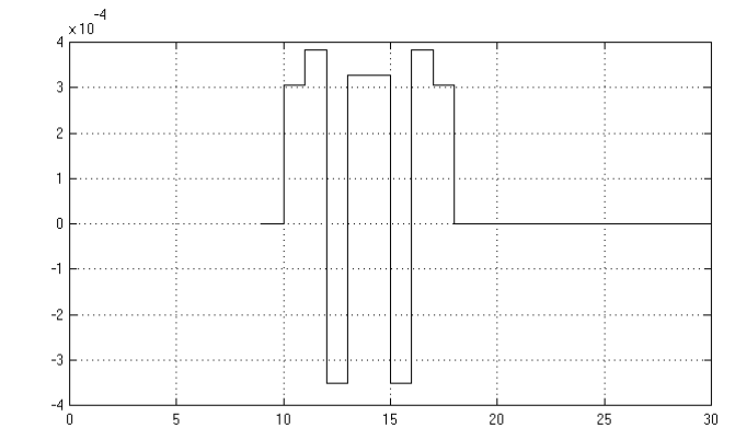
Figure 16: Transposed Form FIR Filter Quantization Error
