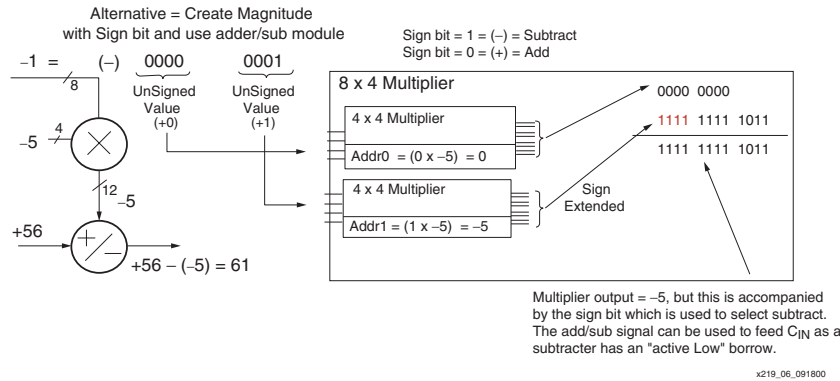
Figure 6: KCM Implementation with Add/Subtract Module
