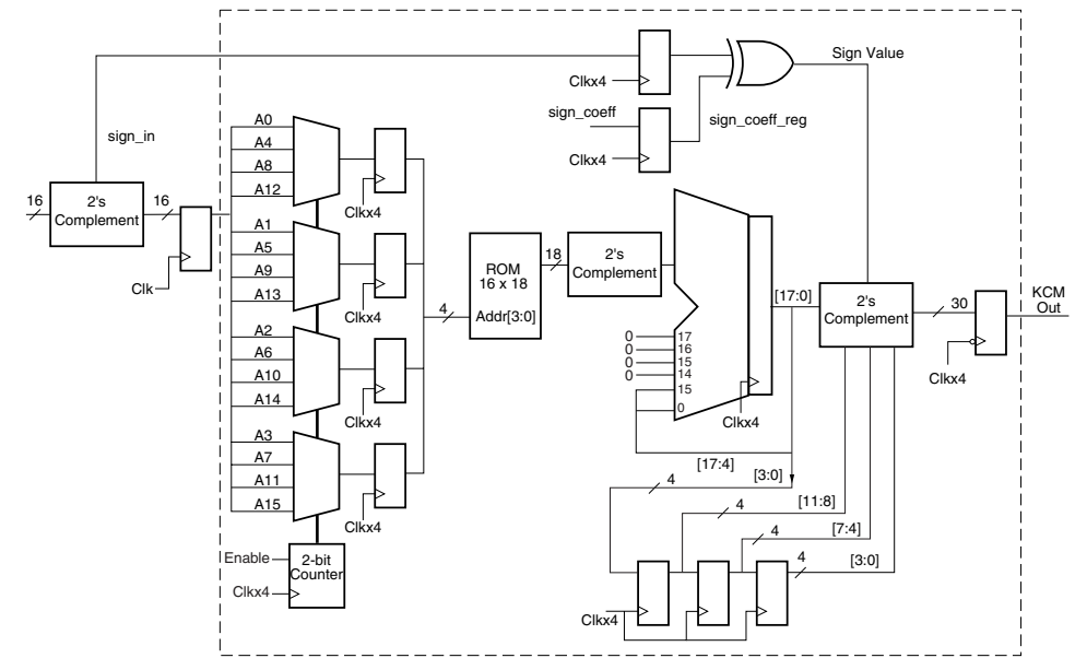
Figure 7: Multicycle KCM implementation
