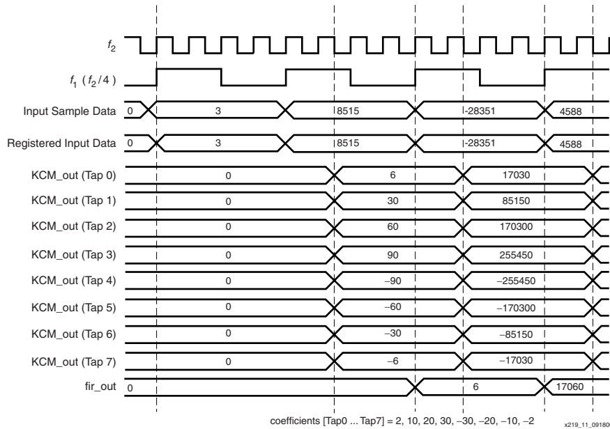
Figure 11: Simulation Waveform
