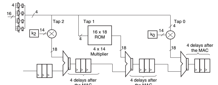
Figure 10: Optimized Transposed Form FIR Filter
