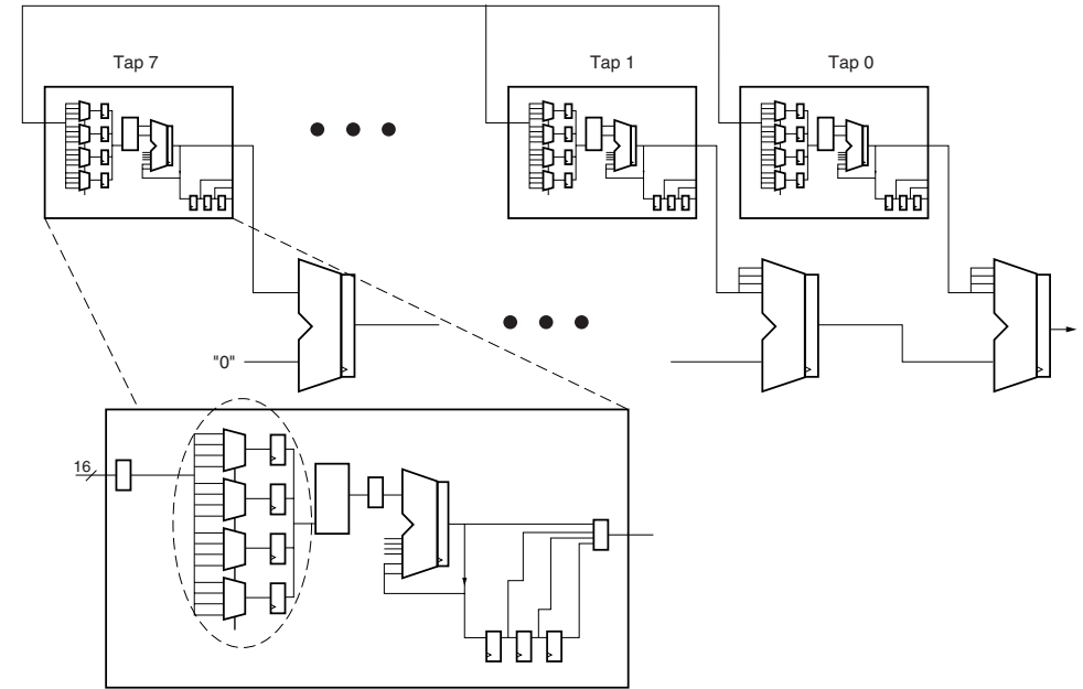
Figure 9: Transposed Form FIR Filter with Eight Taps
