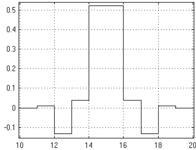
Figure 13: Traditional FIR Filter Impulse Response
