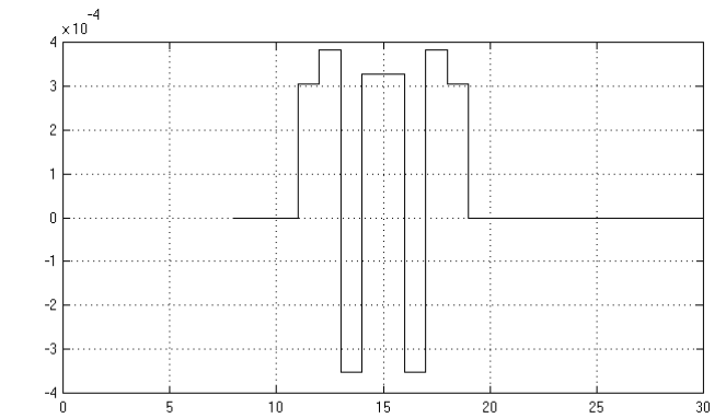
Figure 14: Traditional FIR Filter Quantization Error
