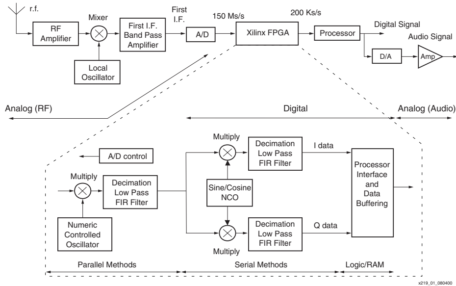
Figure 1: Filter Applications: Communication Receiver
