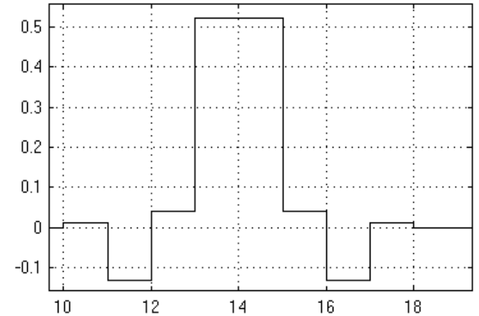
Figure 15: Transposed Form FIR Filter Impulse Response
